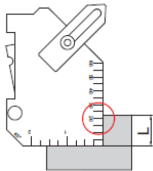
length
