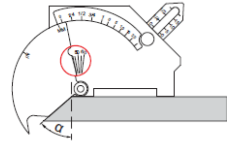
angle of preparation
