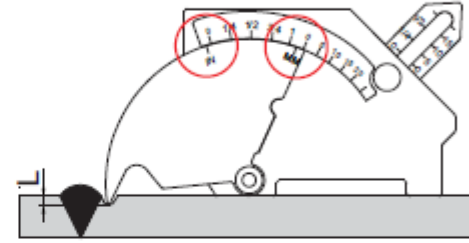
undercut depth
