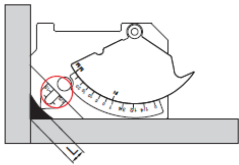
fillet weld throat size
