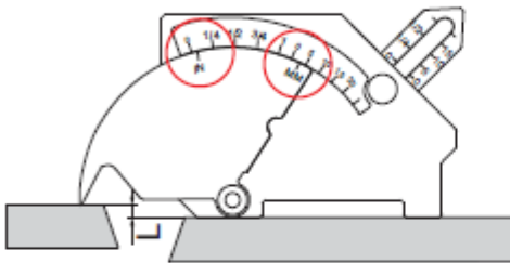
misalignment (high-low)
